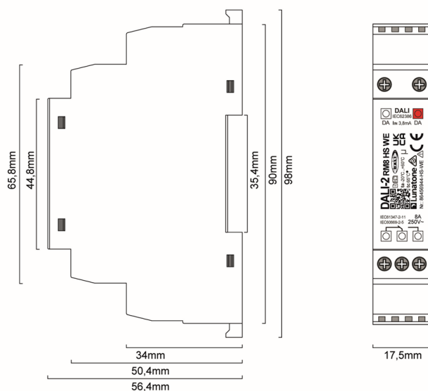
dimensions RM8 HS WE
