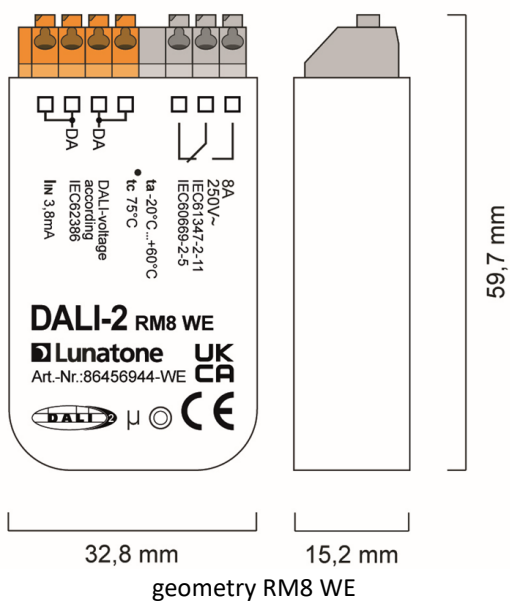
geometry RM8
