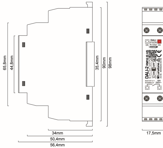
dimensions RM16 IS HS
