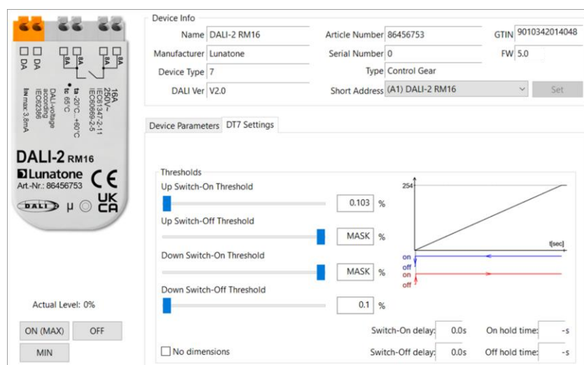
Figure 2 DALI Cockpit tab: DT7 settings
