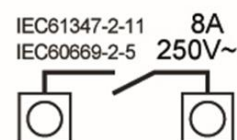
connection plan RM8 HS
